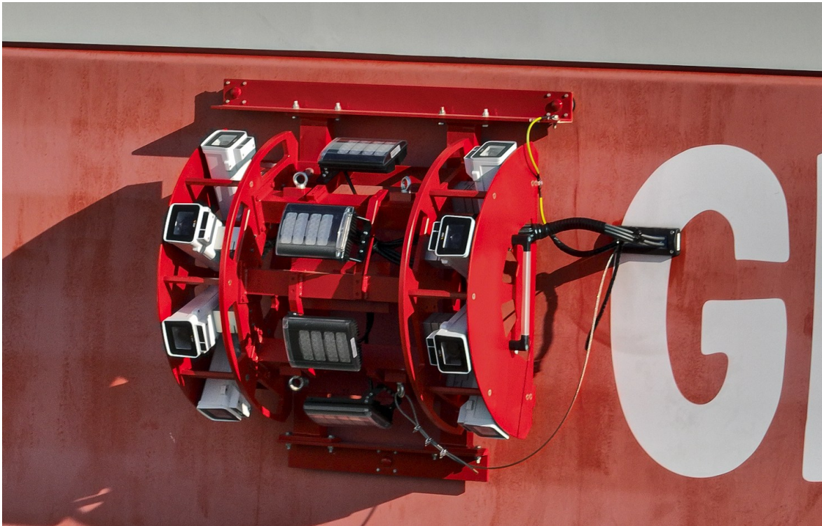
Figure 3-5 The AVES Offshore HPC system, consisting of four stereo-vision camera pairs and infrared light sources to facilitate bird detection at night.
